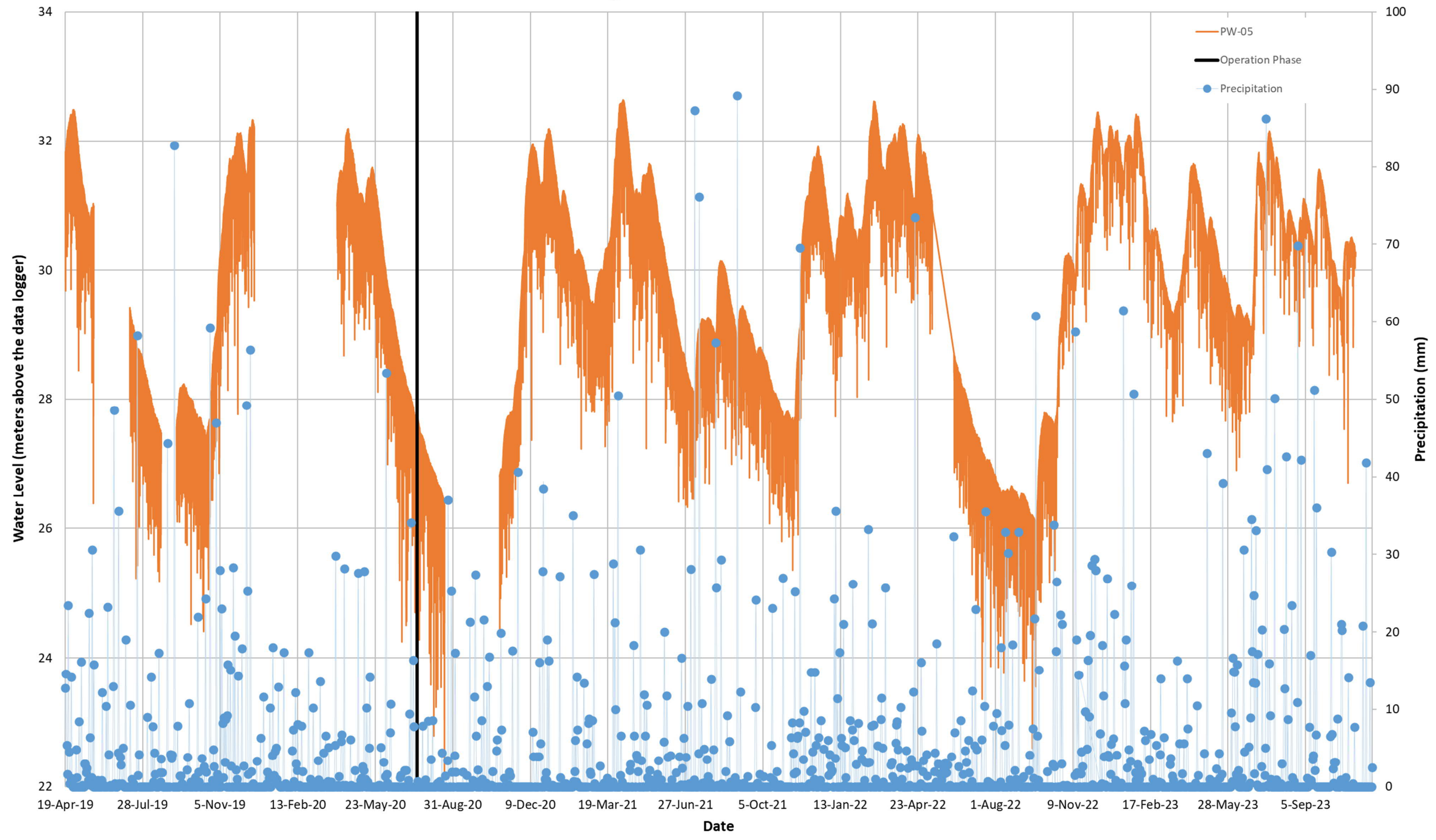
Figure 5: PW-05 Water Levels
