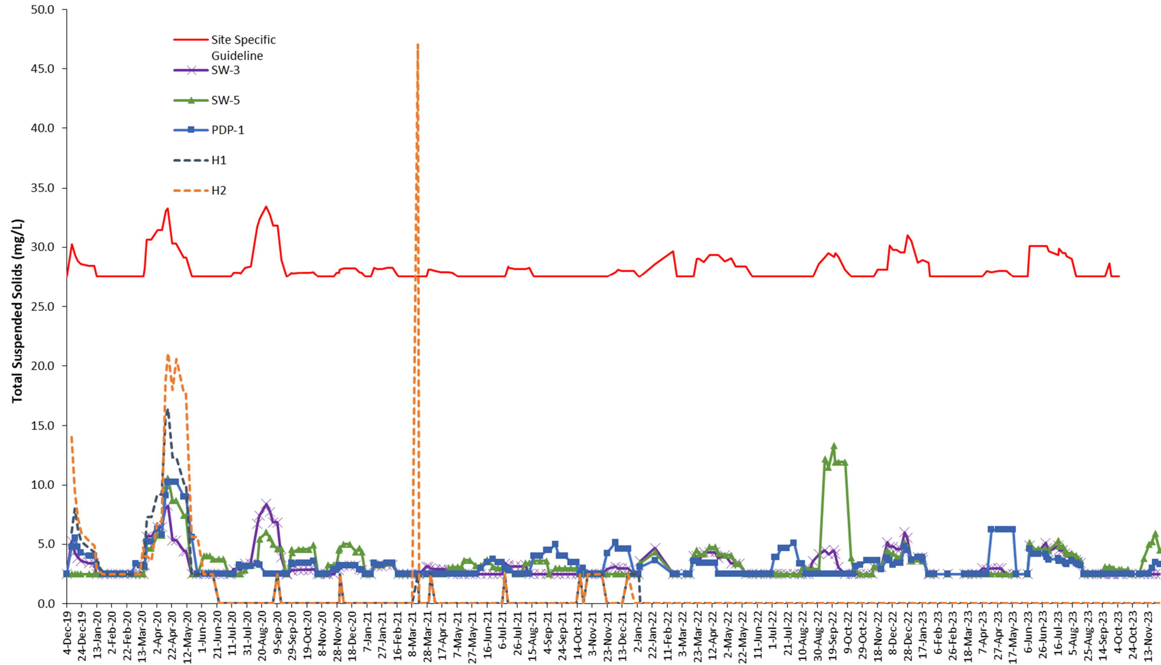
Figure 2: TSS Monthly Average
