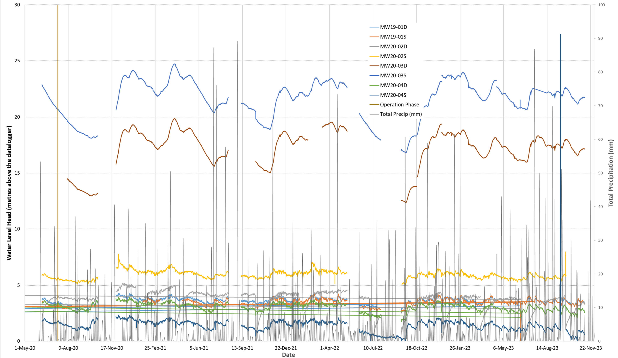
Figure 3: Upham East - Perimeter Monitoring Water Levels
