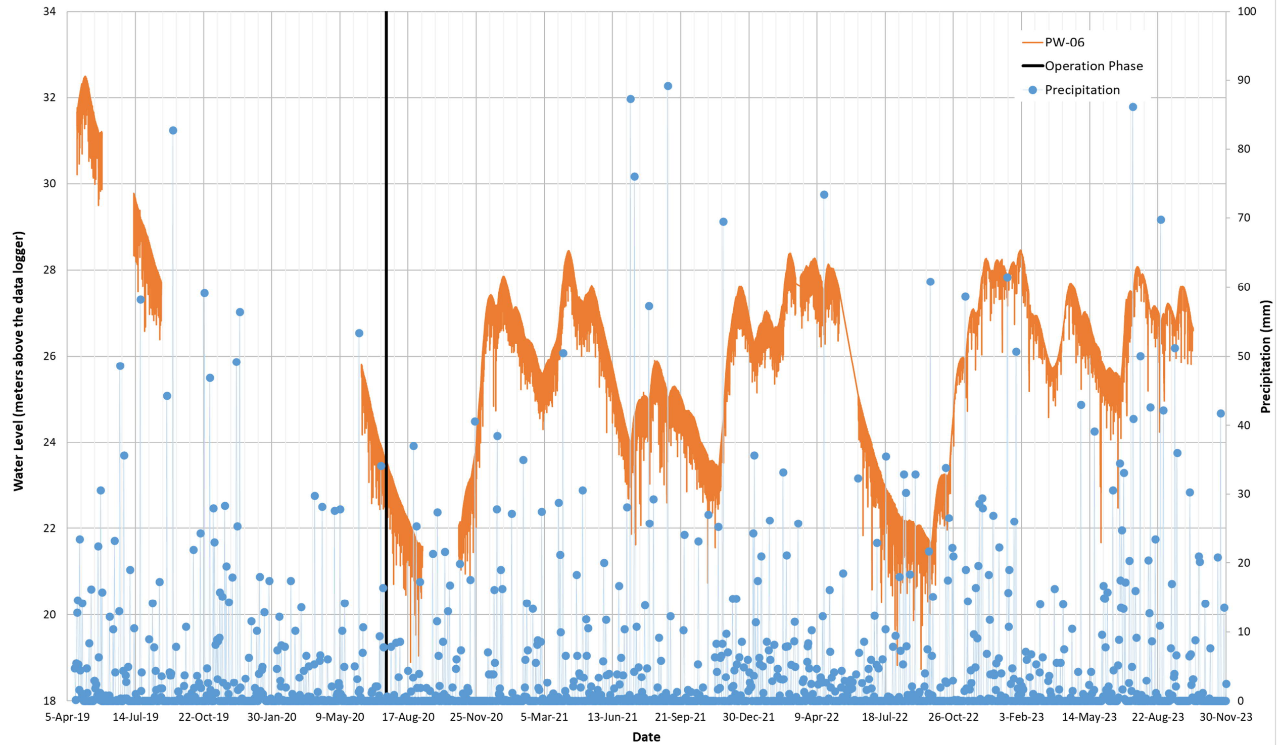
Figure 6: PW-06 Water Levels
