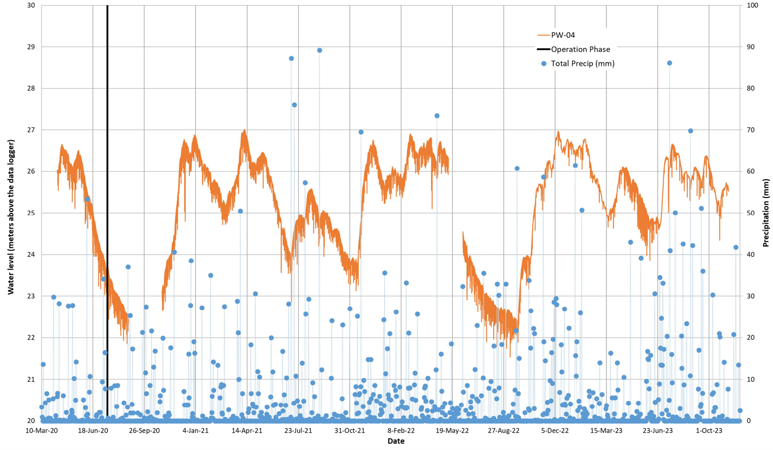
Figure 4: PW-04 Water Levels
